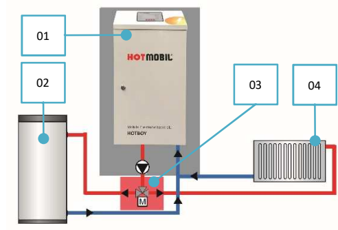
Figure 8: Hydraulics schematic – hot water reservoir
